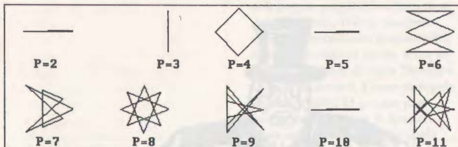
PROGRAMMA NO. 8a-3 T=3, U=5
