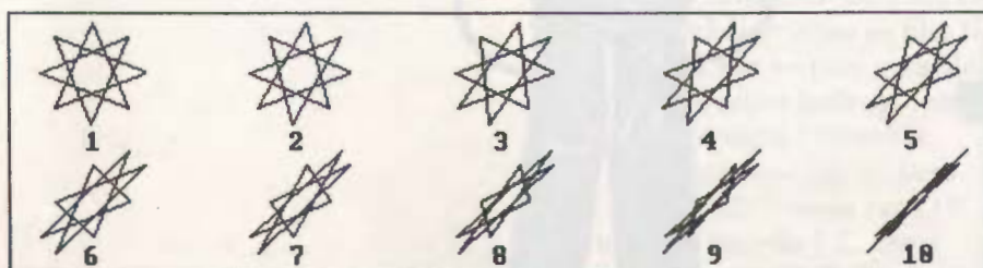
PROGRAMMA No. 8a-4 FX=FX+PI/20 P=8 T=3, U=5
